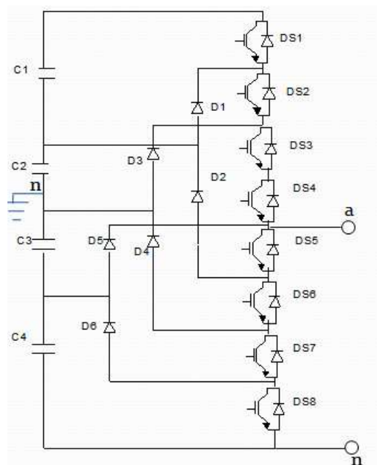
Fig. 2 Five Level Diode Clamped Multilevel Inverter
