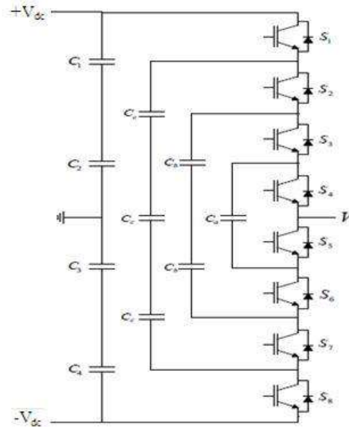
Fig. 3 Five Level Flying Capacitor Multilevel Inverter
