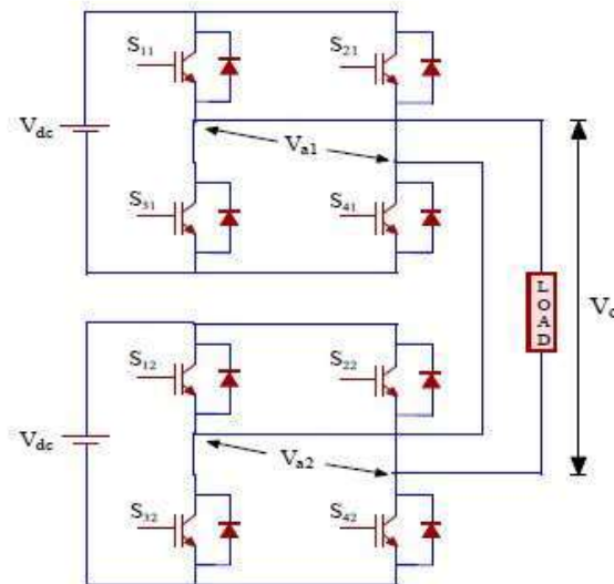
Fig. 1 Five Level cascaded H-bridge Multilevel Inverter
